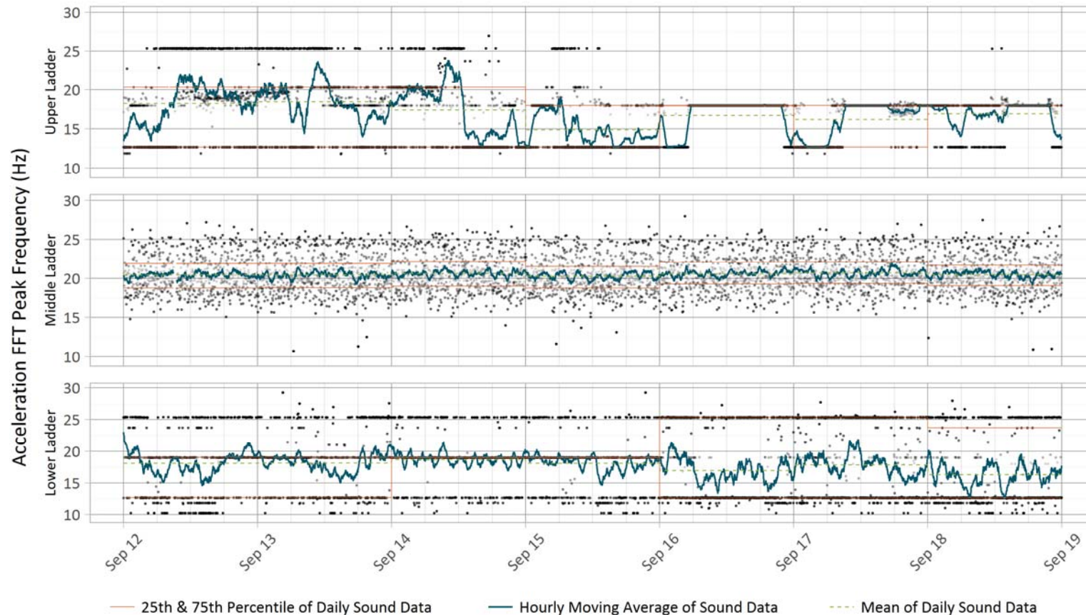
Figure 2 Acceleration Peak Frequencies Measured by Triaxial Accelerometers for Week 37
