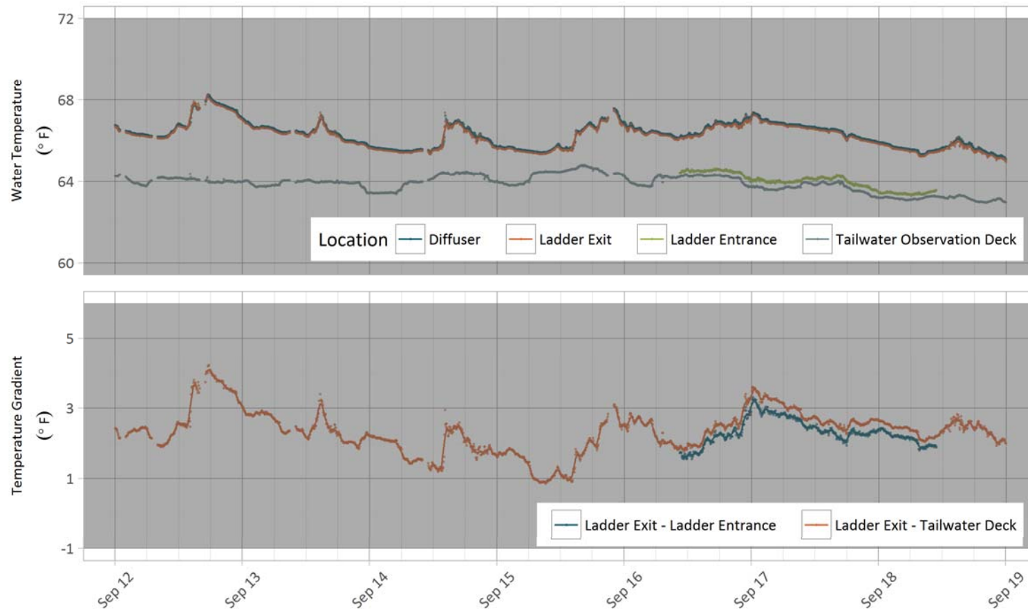
Figure 3 Water Temperatures in the Fish Ladder for Week 37
