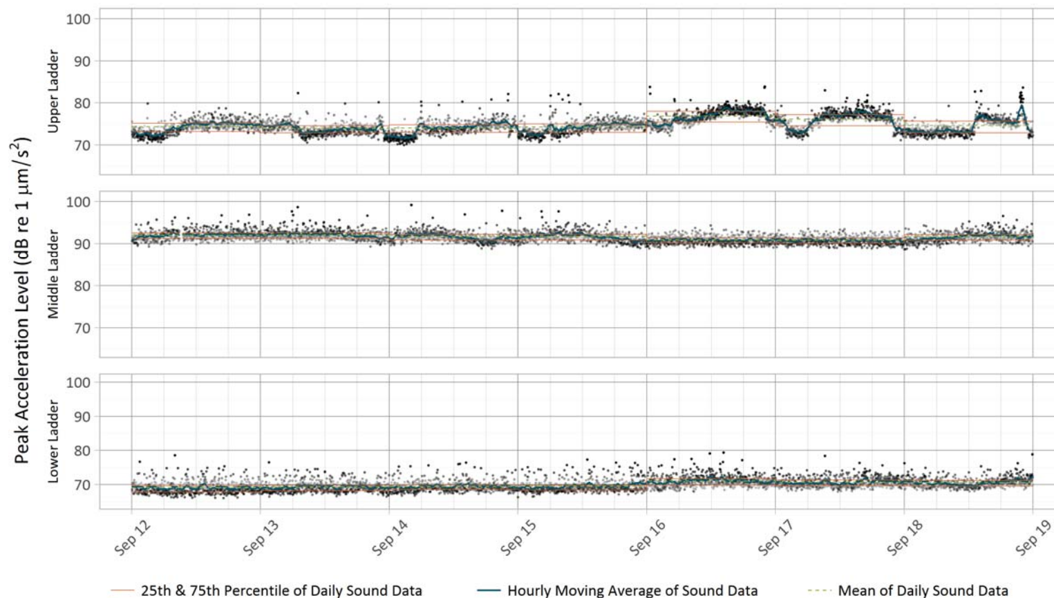
Figure 1 Peak Acceleration Levels Measured by Triaxial Accelerometers for Week 37
